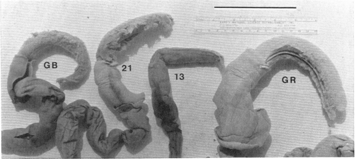
Figure 4. Anterior regions of the specimens of four populations of Riftia —Guaymas Basin (GB), 21 degrees North (21), 11 to 13 degrees North (13) and the Galápagos Rift (GR). Note differences in relative lengths of obturacula and vestimenta (scale bar is 10 centimeters).
